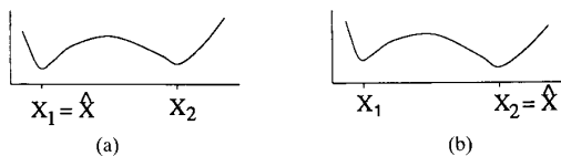
Fig. 2. This figure illustrate how small changes in a nonconvex function can result in large changes in the location of the function's minimum value.
