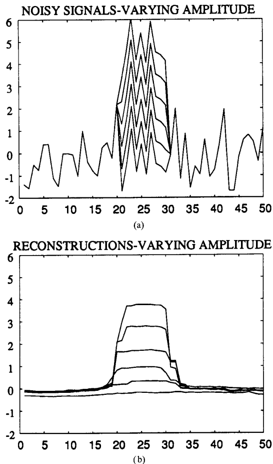
Fig. 6. MAP estimates using GGMRF prior with p = 1 , \lambda = 5 . (a) Noisy square pulses with amplitudes of 0, 1, 2, 3, 4, and 5. Each contains additive white Gaussian noise of unit variance. (b) Resulting MAP estimates using GGMRF prior with p = 1 , \lambda = 5 , and b_{s,r} = 1 for adjacent points. Optimization was performed using 10^4 full iterations of simulated annealing.
