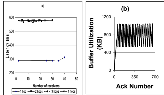
Figure 6. Evaluation of TRAM in error-free case
