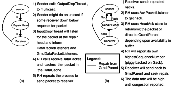
Figure 4. TRAM++ implementation for (a) upstream and (b) downstream message processing with message errors
