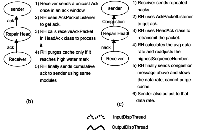
Figure 2. TRAM message processing (a) downstream with no errors, (b) upstream with no errors, (c) upstream with message, node or link errors
