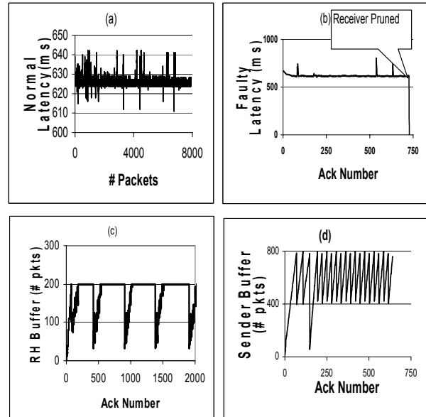
Figure 10. Evaluation of TRAM++ under message drop rate of 5 out of 50 packets.
