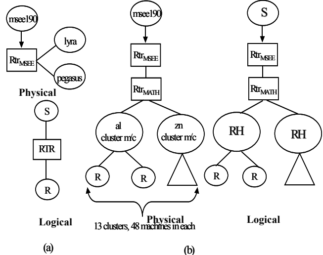
Figure 5. Sample physical and logical configuration for deployment with (a) 2 hops (b) 4 hops between sender & receiver
