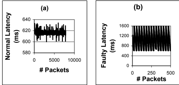
Figure 11. Effect of message delay (1000 ms) on TRAM++ (a) Normal receiver (b) Faulty receiver
