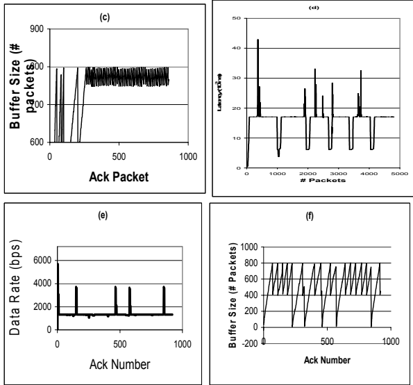
Figure 7. Effect of message drop on TRAM: (a)&(d) Latency for 3 and 5 packets dropped out of 50, (b)&(e) Data Rates, (c)&(f) Buffer Occupancy
