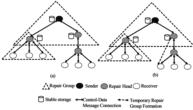
Figure 1. (a) TRAM hierarchical repair tree (from [2]) (b) TRAM++ hierarchical repair tree with temporary reaffiliation
