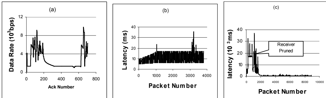
Figure 8. Effect of message delay on TRAM: (a)-(b) Delay of 8000 ms, no pruning; (c) Delay of 10000 ms, pruning.
