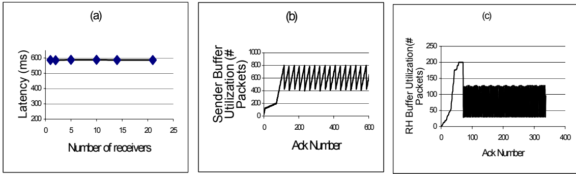
Figure 9. Evaluation of TRAM++ in error-free case: (a) Receiver latency (b) Sender buffer utilization and (c) Repair Head buffer utilization for 27 receivers
