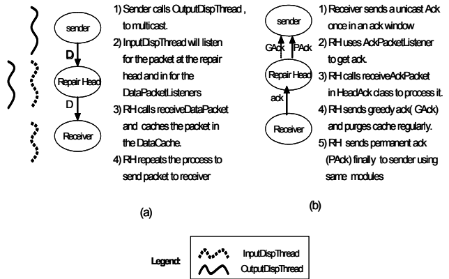
Figure 3. TRAM++ implementation for (a) upstream and (b) downstream message processing with no errors
