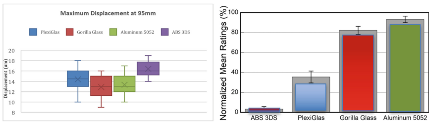
Fig. 3. Variance in displacement for CWI in um (left) and perceived differences between signals at points A and B (right) through constructive wave interference (virtual exciter) on the 3 + 1 waveguides
