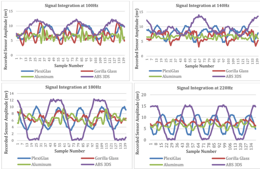
Fig. 4. 100 Hz (top left), 140 Hz (top right), 180 Hz (bottom left) and 220 Hz (bottom right) signals recorded at 95 mm from the source actuator to illustrate distortion/attenuation in the 4 surfaces
