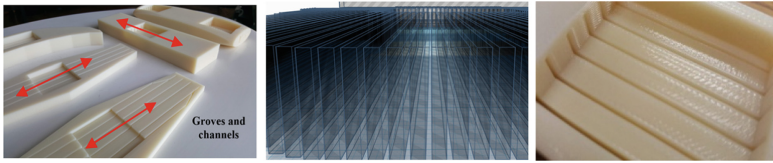
Fig. 1. Multiple iterations of the 3D-printed waveguides.
