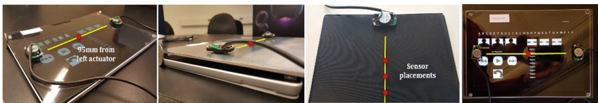
Fig. 2. Measuring wave propagation and virtual exciters within the 3 + 1 surfaces.
